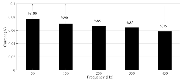
Figure 5. Harmonic distribution of MO current.
