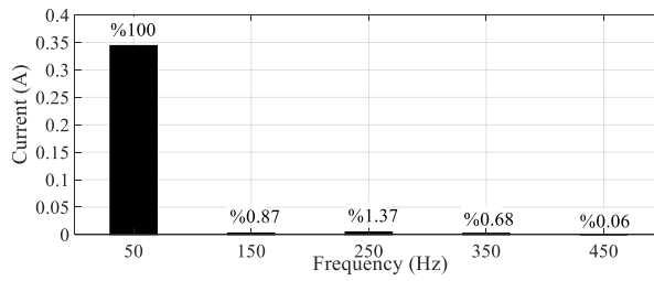
Figure 4. Harmonic distribution of HL current.
