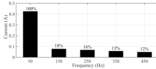
Figure 7. Harmonic analysis of MO & HL current.
