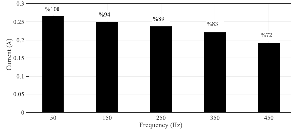
Figure 6. Harmonic analysis of MO & LC current.
