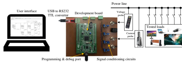
Figure 1. Experimental setup of the real-time load identification system.
