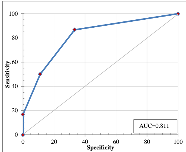
1 Table-3: Sensitivity and Specificity of pH at different cut-off values based on Receiver Operator
