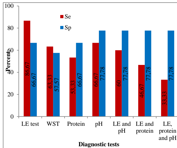
Figure-4: Sensitivity and Specificity of diagnostic tests in comparison to Endometrial Cytology.
