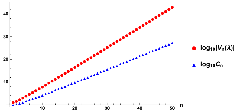
Figure 3: The comparison of the absolute value of the numbers V_n(\lambda) (represented by red filled circles) with the Catalan numbers C_n (represented by blue filled triangles) by plots of their logarithms with base 10 versus n while \lambda = \frac{1}{2} .
