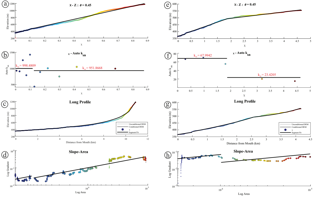
Figure S3. Topographic characteristics of the main channel profile of the drainage basins 12 and 14. a and e) Elevation-chi ( \chi ) plot of channel profile and transient stage of the profiles. b and f) Auto k_{sn} -chi ( \chi ) plot shows the main steepness variations along the profile. c and g) Longitudinal profile of the main channel and its morphologic properties. d and h) Logarithmic slope-area of the channel and steepness based segmentation.
