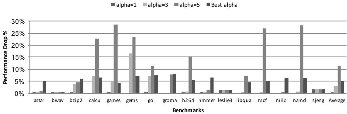
Figure 3. Percentage of performance drop of ShapeShifter compared to baseline out-of-order processor for various alpha thresholds. The best alpha represents the best performing alpha value for each benchmark, respectively.
