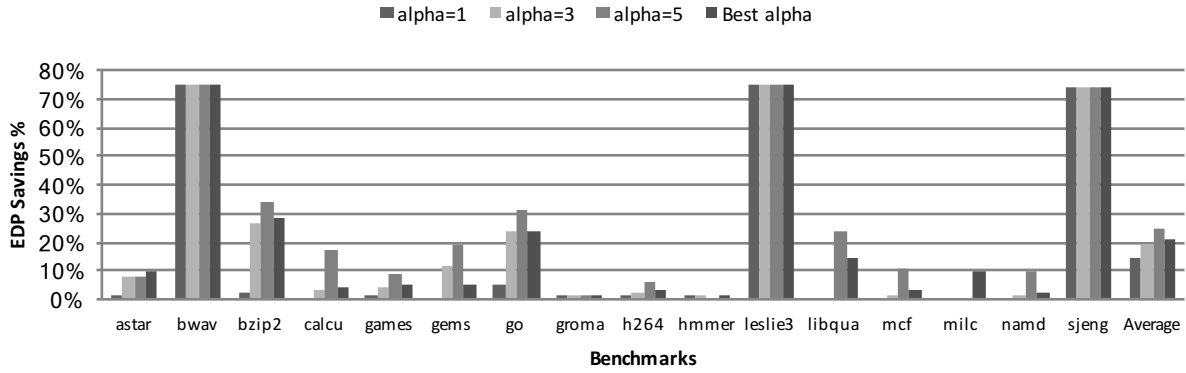
Figure 5. Percentage of EDP savings of ShapeShifter compared to baseline out-of-order processor for various alpha thresholds. The best alpha represents the best performing alpha value for each benchmark, respectively.
