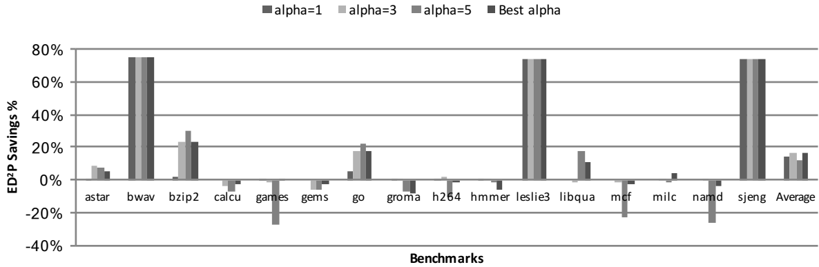
Figure 6. Percentage of ED 2 P savings of ShapeShifter compared to baseline out-of-order processor for various alpha thresholds. The best alpha represents the best performing alpha value for each benchmark, respectively.
