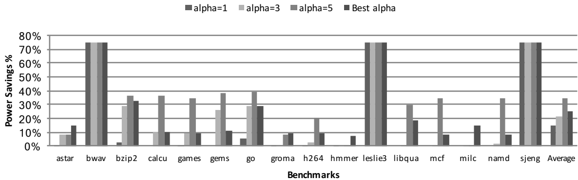
Figure 4. Percentage of power savings of ShapeShifter compared to baseline out-of-order processor for various alpha thresholds. The best alpha represents the best performing alpha value for each benchmark, respectively.
